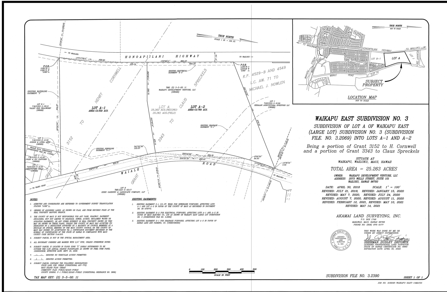
Figure 6. Subdivision Plan for No. 3 (Lots A-1 and A-2)
