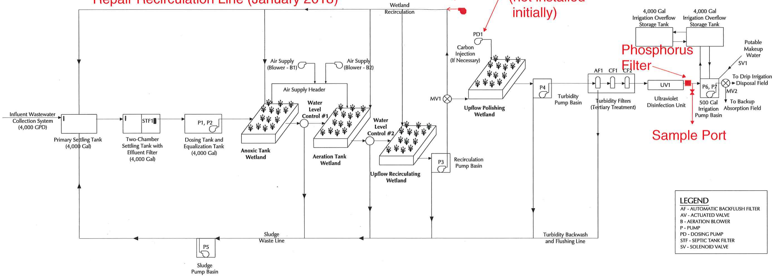
Process Flow Diagram Scale: None
