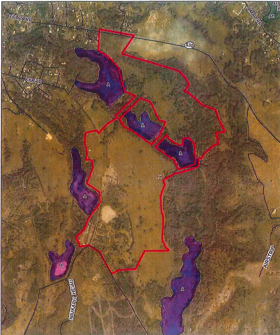
FIGURE 9 Flood Hazard Zones Lawai Solar and Storage Project Koloa, Kauai, Hawaii
