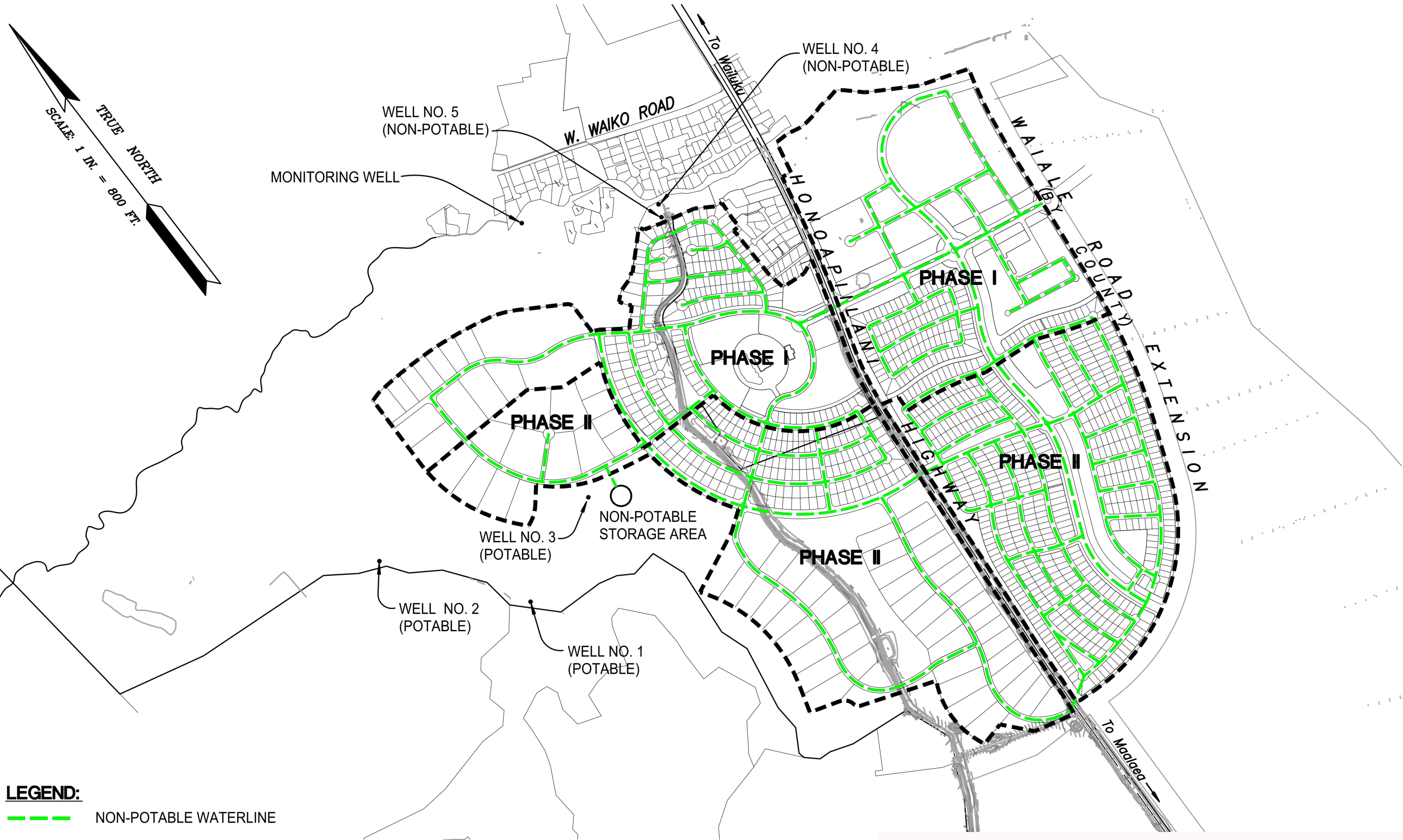
Figure 33, B: Conceptual Non-Potable Water Phasing Diagram
