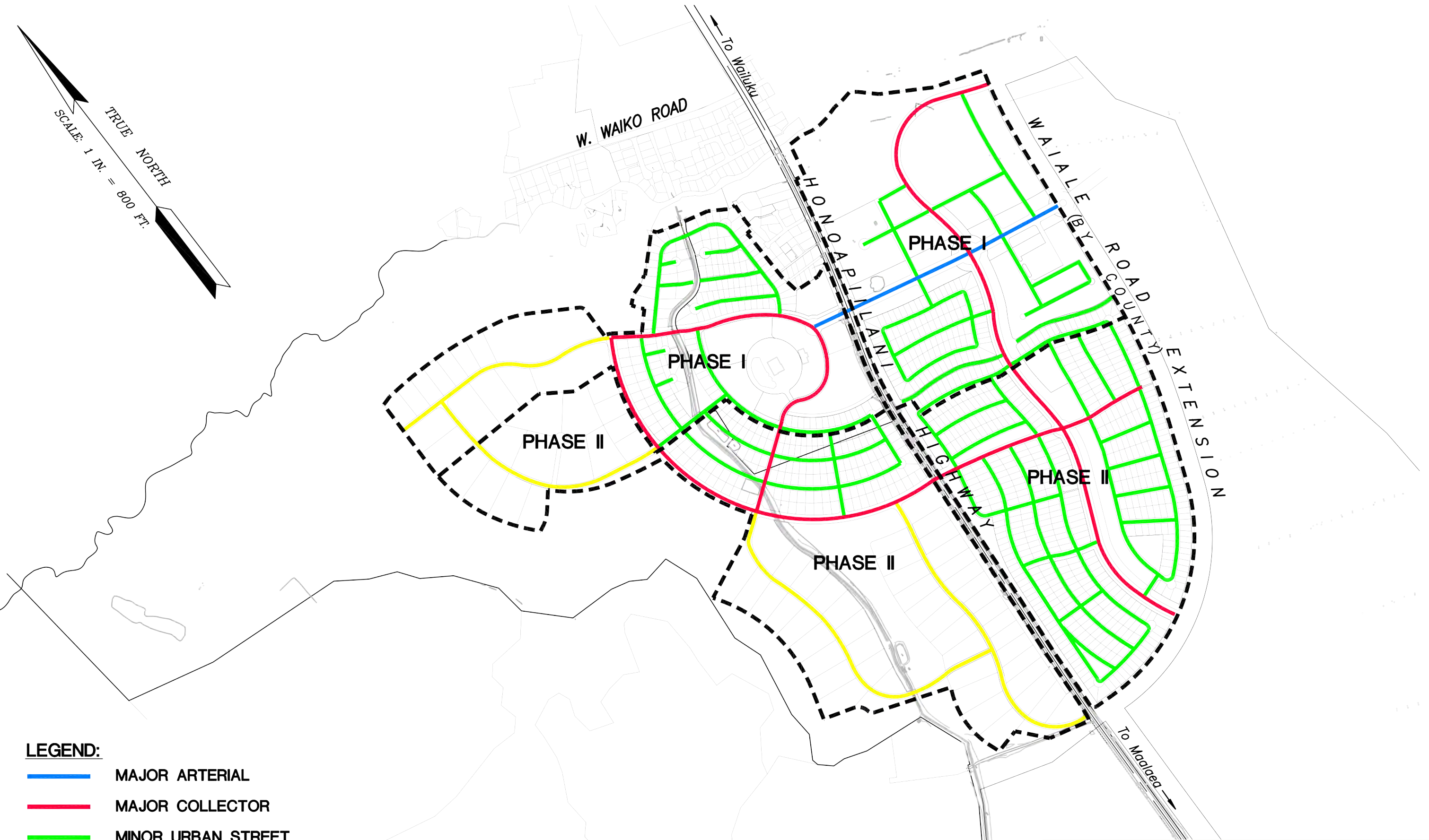
Figure 31 Conceptual Roadway Improvement Phasing Diagram
