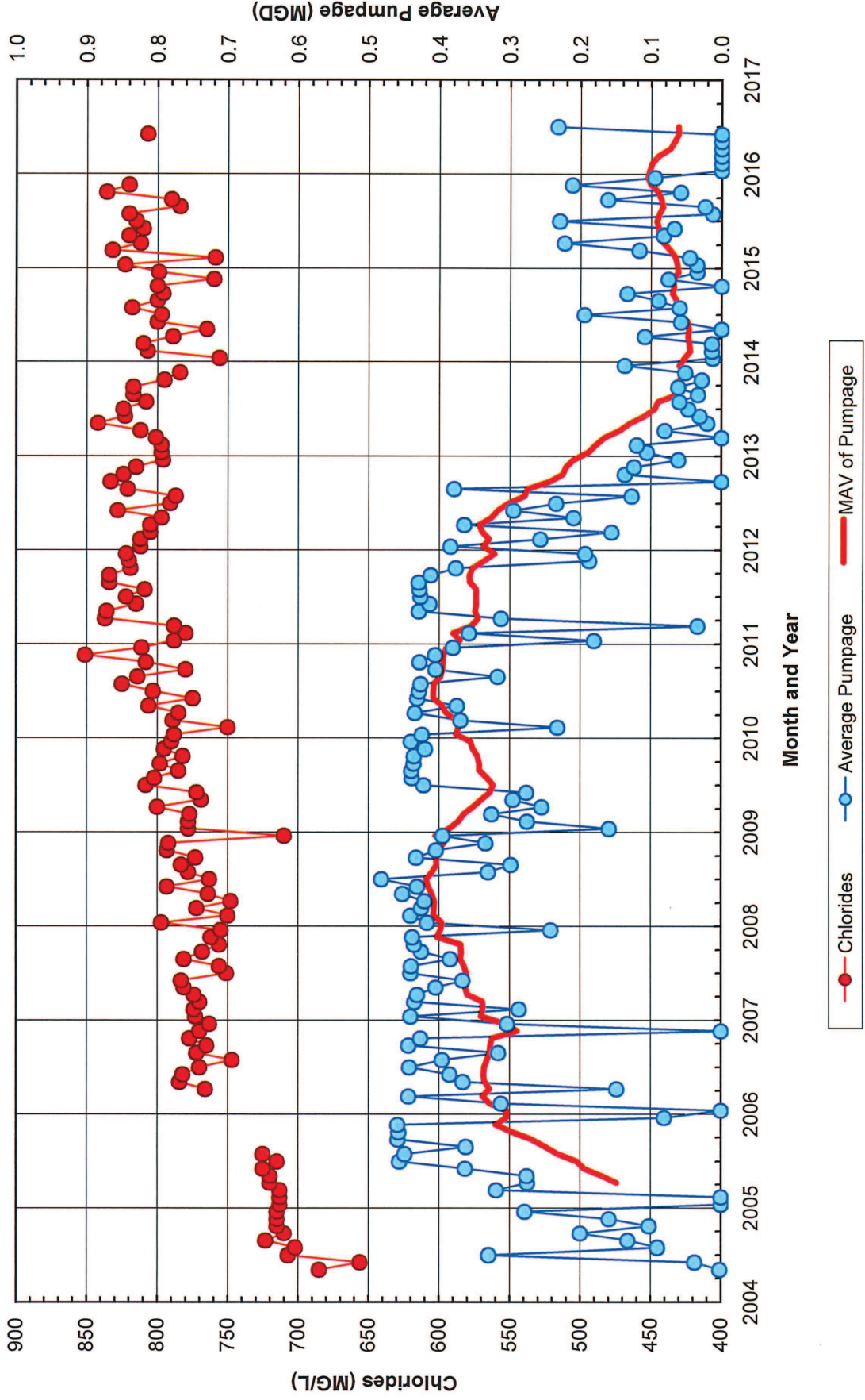
Chlorides and Pumpage of Lanai Well 14 Since its Use Started in May 2004
