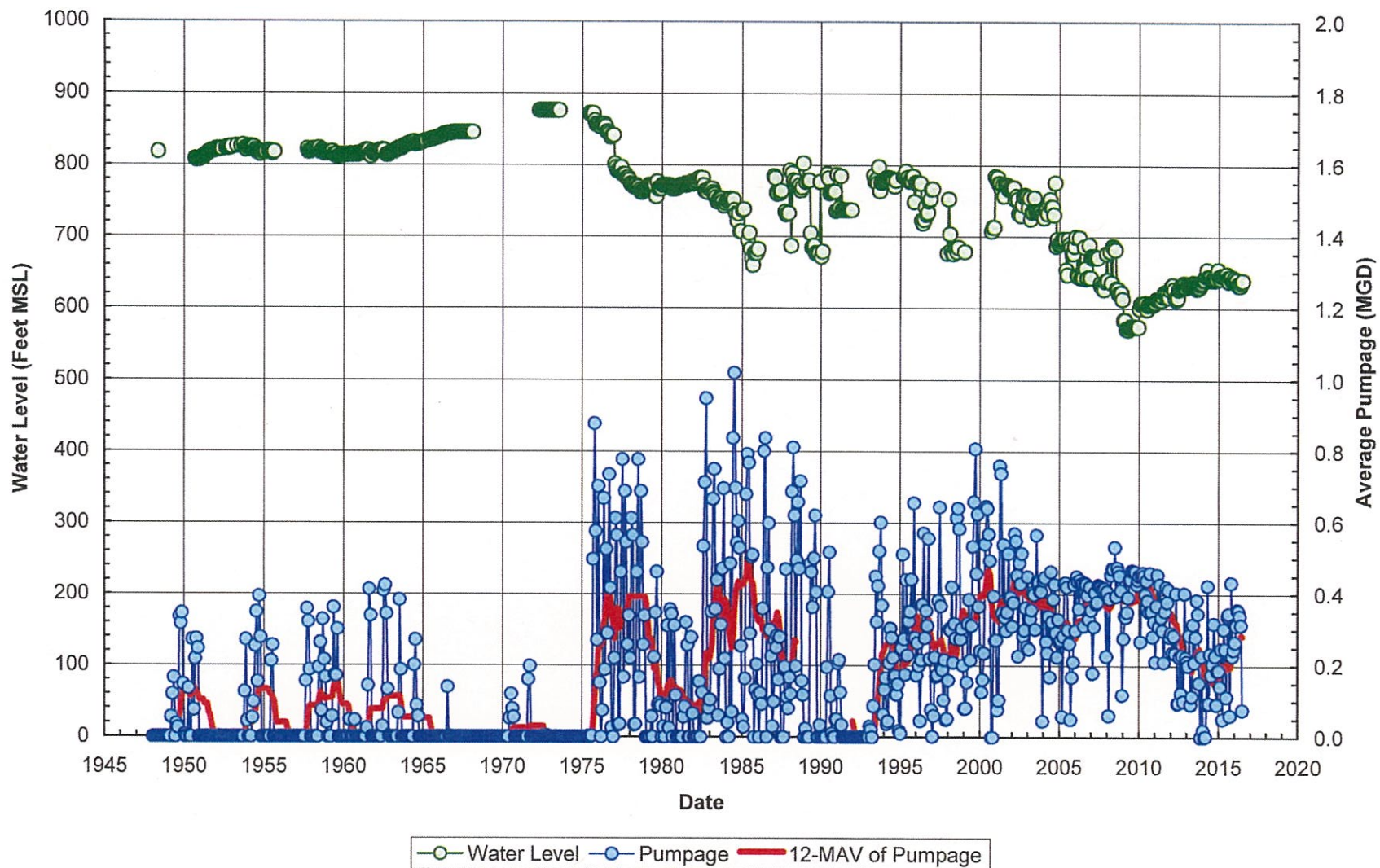
Water Level and Pumpage of Well 1, 1948 to 2016
